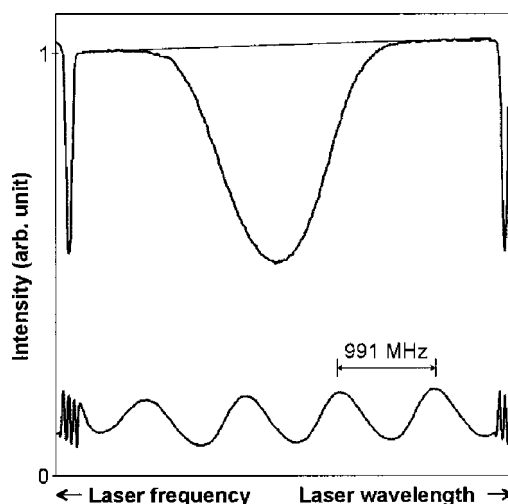
Fig. 3. Raw data obtained in an absorption recording of the 4s\ ^2S_{1/2}-4p\ ^2P_{1/2} potassium transition. Note the increasing laser output over the scan, but the quasi-linear frequency sweep as evidenced by equidistant Fabry-Perot fringes. The signals associated with the retrace at the end of the saw-tooth sweep are also evident.
